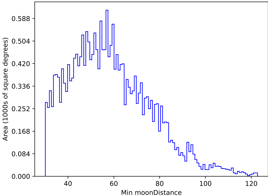
too_elab_r128_d3_gz_v3.4_10yrs All sky u band: Min moonDistance
