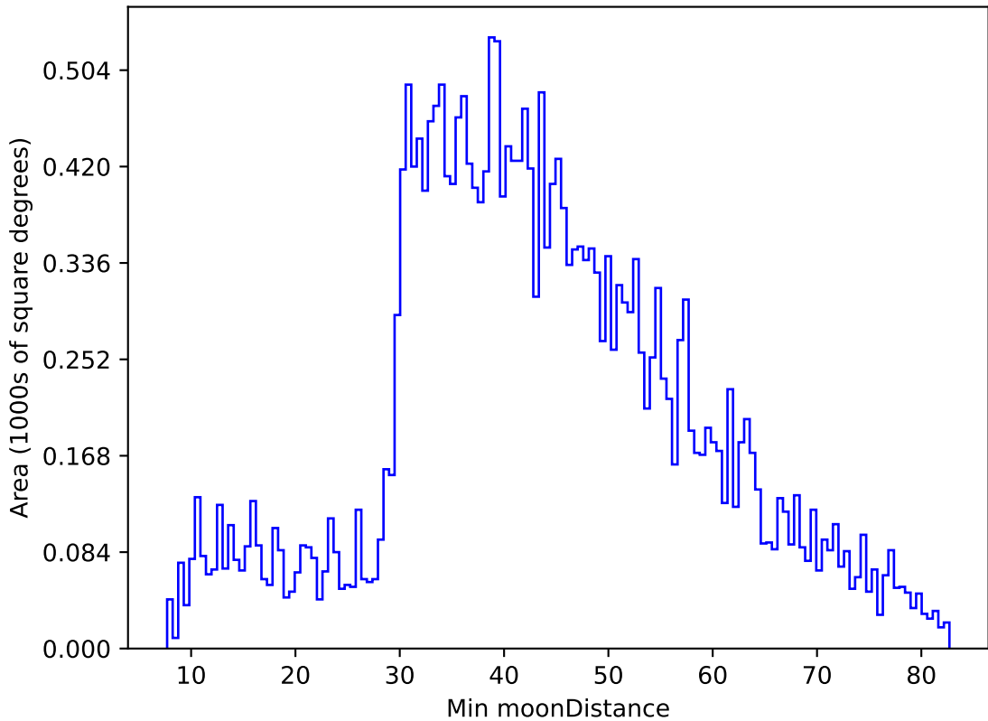
too_elab_r128_d3_gz_v3.4_10yrs All sky g band: Min moonDistance
