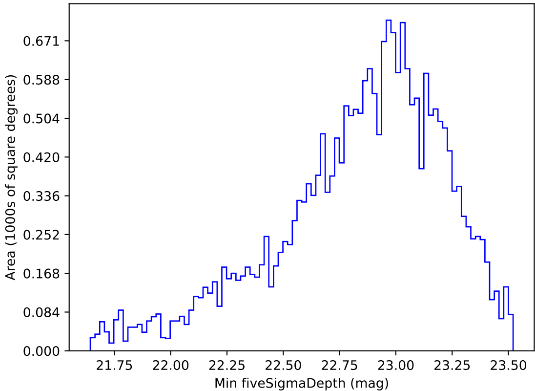
too_elab_r128_d3_gz_v3.4_10yrs Yr 1 u band: Min fiveSigmaDepth
