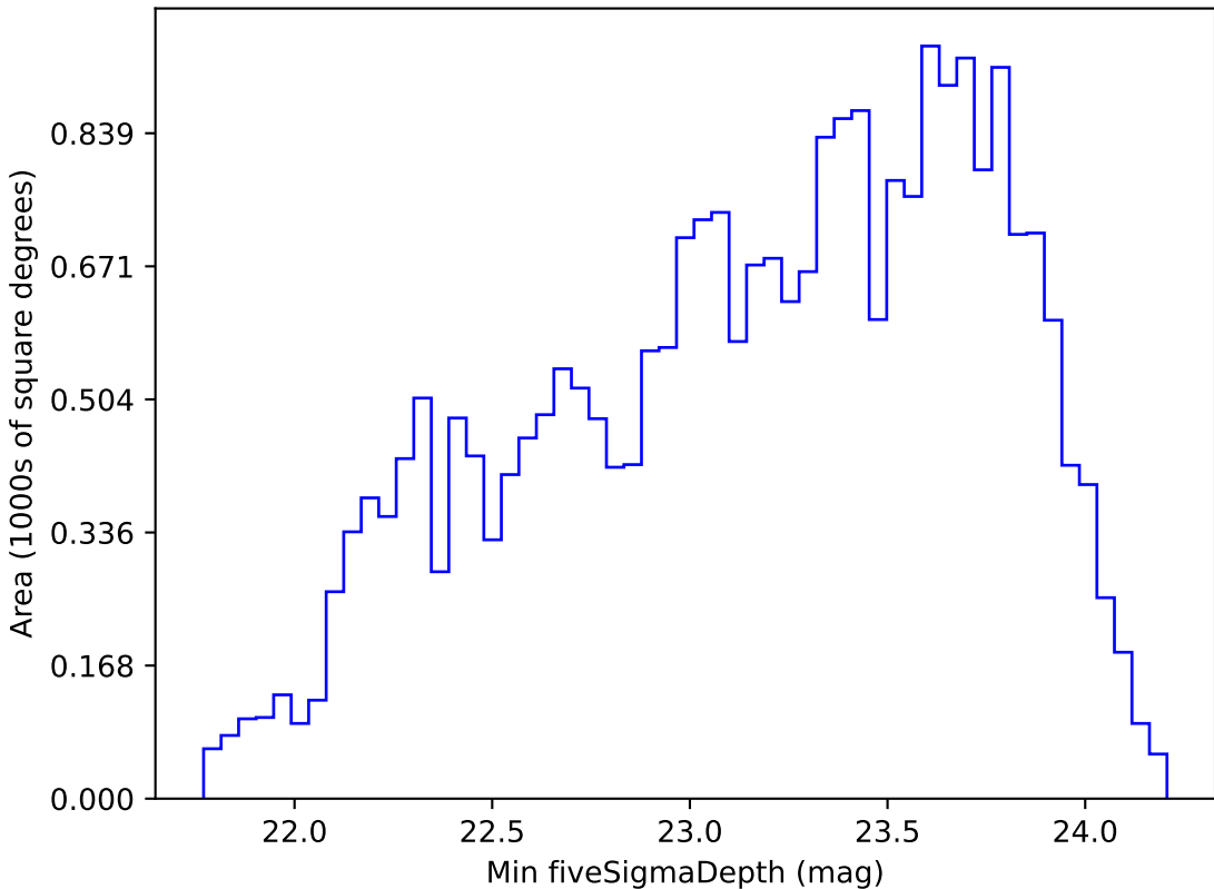
too_elab_r128_d3_gz_v3.4_10yrs Yr 1 r band: Min fiveSigmaDepth
