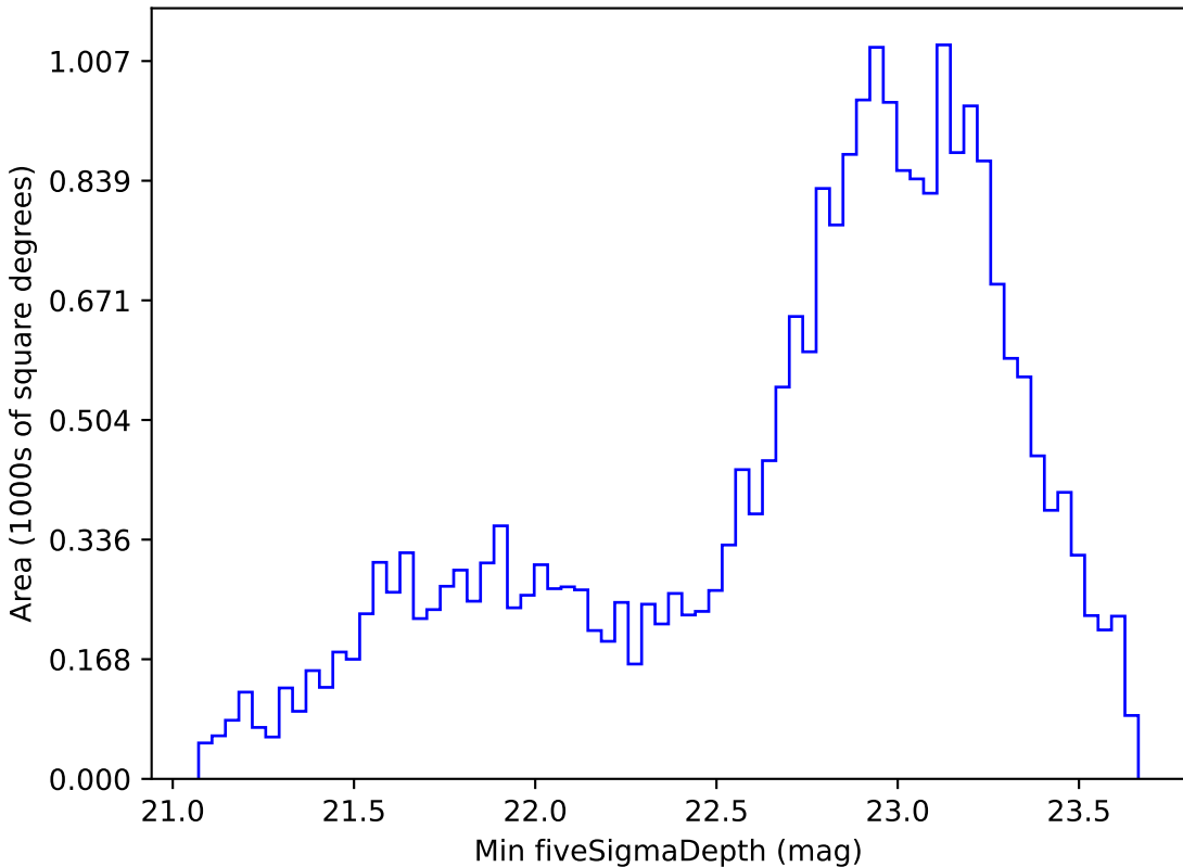
too_elab_r128_d3_gz_v3.4_10yrs Yr 1 i band: Min fiveSigmaDepth
