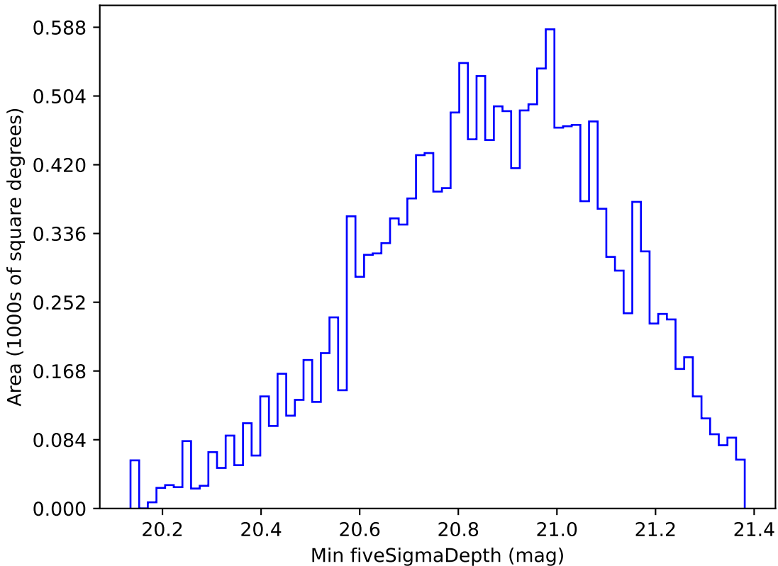
too_elab_r128_d3_gz_v3.4_10yrs WFD y band: Min fiveSigmaDepth
