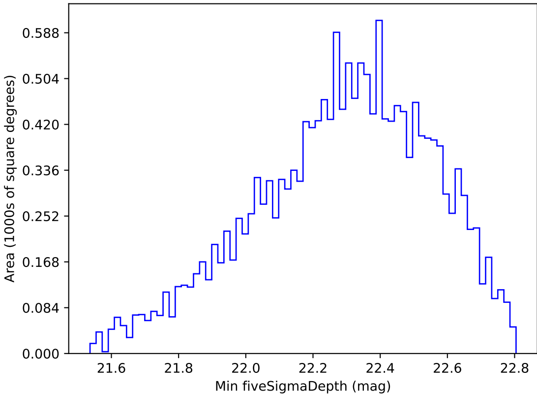
too_elab_r128_d3_gz_v3.4_10yrs WFD u band: Min fiveSigmaDepth
