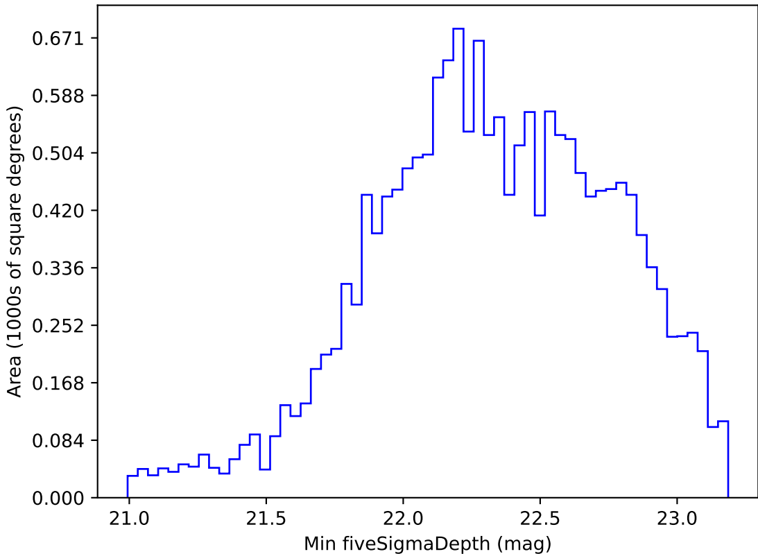
too_elab_r128_d3_gz_v3.4_10yrs WFD r band: Min fiveSigmaDepth
