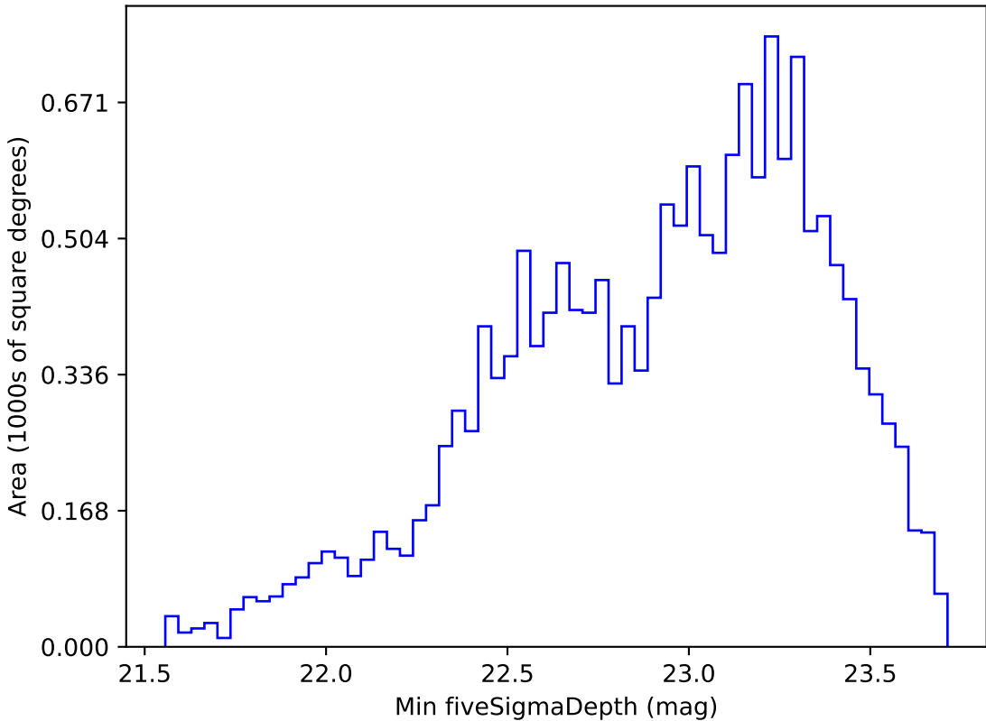
too_elab_r128_d3_gz_v3.4_10yrs WFD g band: Min fiveSigmaDepth
