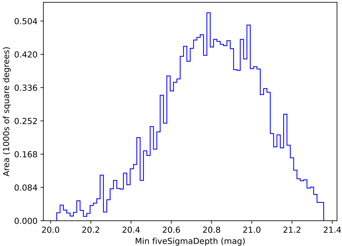
too_elab_r128_d3_gz_v3.4_10yrs WFD all bands: Min fiveSigmaDepth
