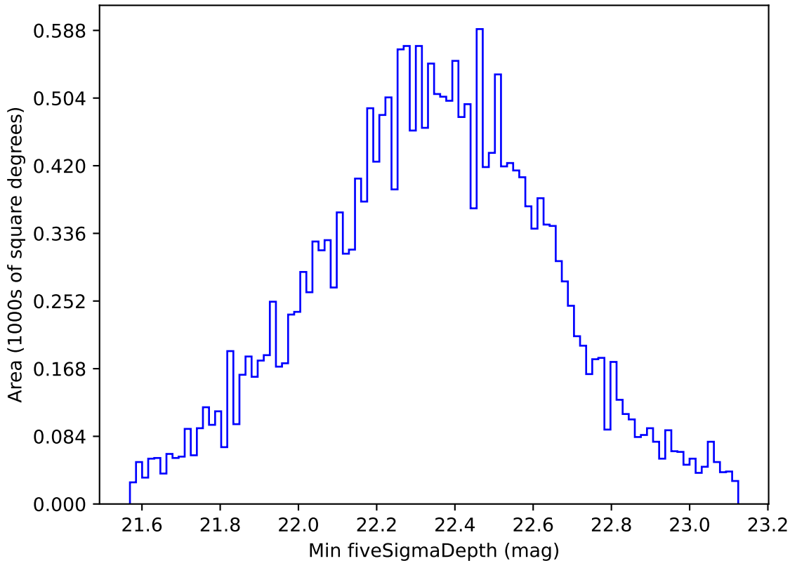
too_elab_r128_d3_gz_v3.4_10yrs All sky u band: Min fiveSigmaDepth
