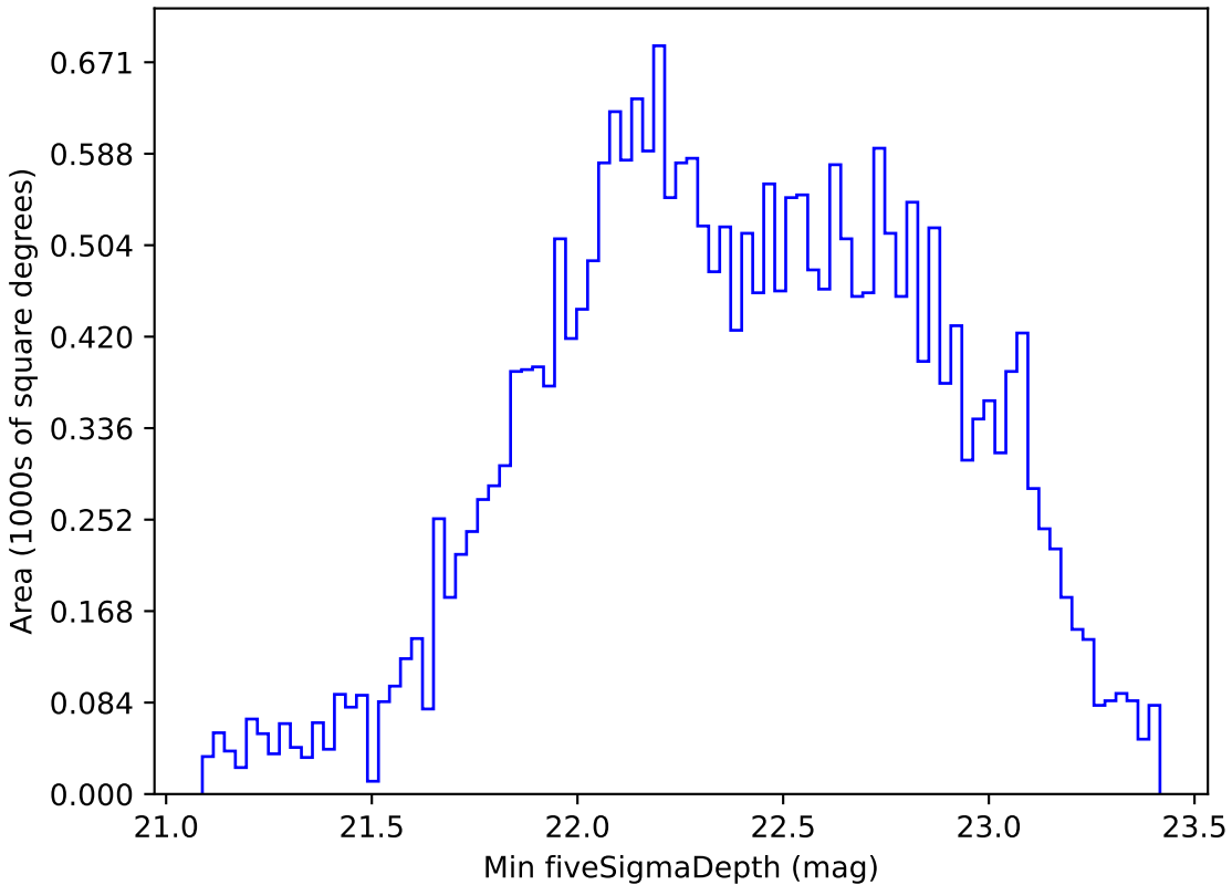
too_elab_r128_d3_gz_v3.4_10yrs All sky r band: Min fiveSigmaDepth
