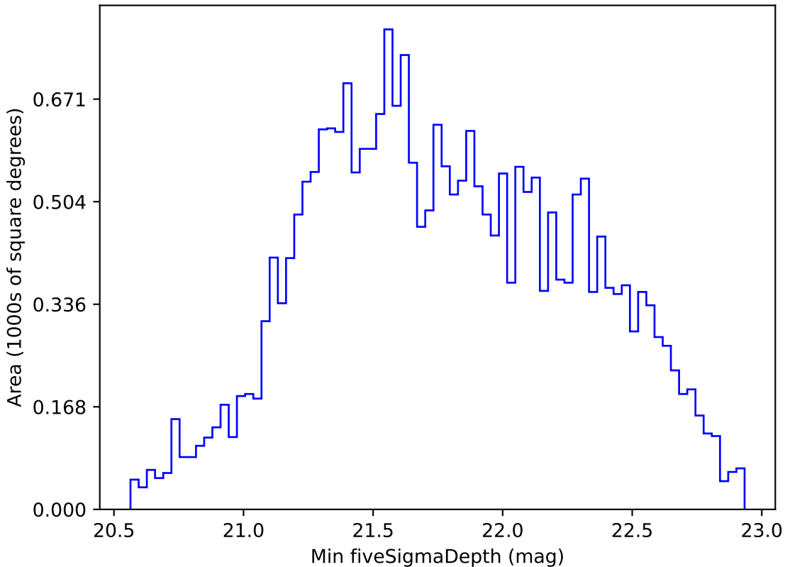
too_elab_r128_d3_gz_v3.4_10yrs All sky i band: Min fiveSigmaDepth
