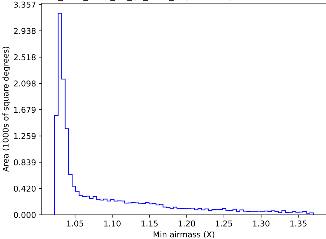
too_elab_r128_d3_gz_v3.4_10yrs WFD y band: Min airmass
