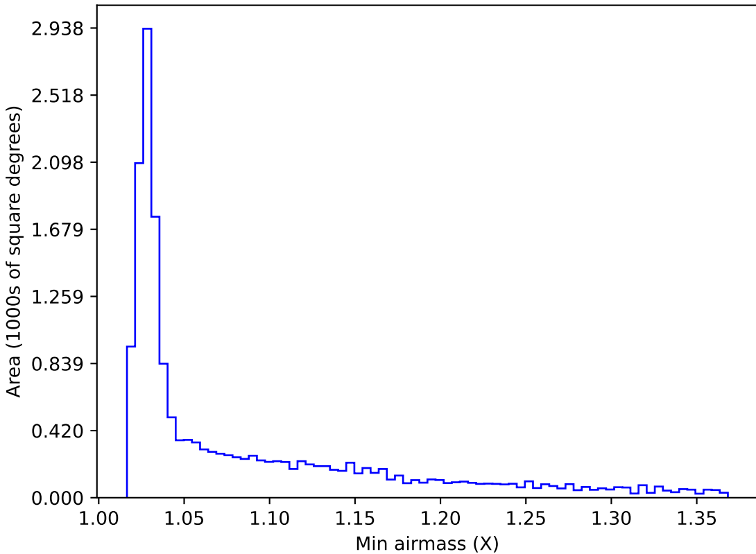
too_elab_r128_d3_gz_v3.4_10yrs WFD r band: Min airmass
