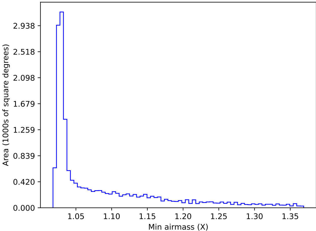
too_elab_r128_d3_gz_v3.4_10yrs WFD i band: Min airmass
