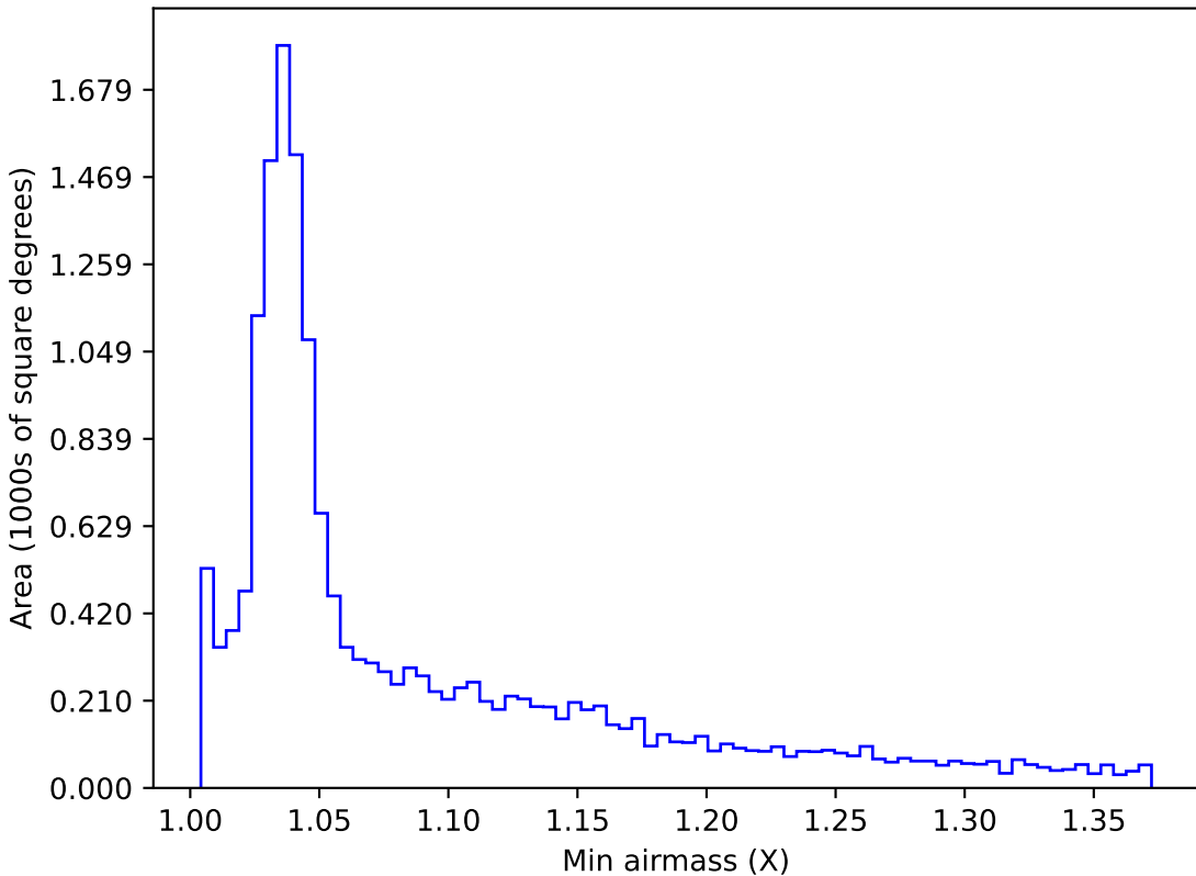
too_elab_r128_d3_gz_v3.4_10yrs WFD g band: Min airmass
