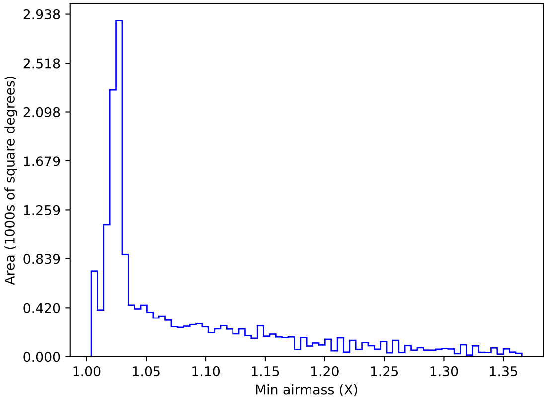
too_elab_r128_d3_gz_v3.4_10yrs WFD all bands: Min airmass
