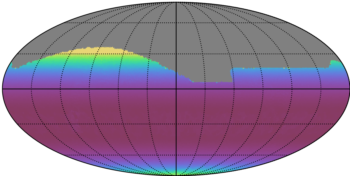
too_elab_r128_d3_gz_v3.4_10yrs All sky r band: Min airmass
