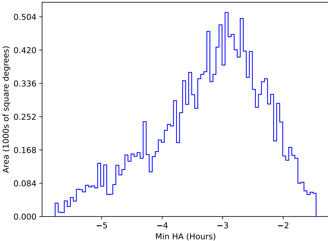
too_elab_r128_d3_gz_v3.4_10yrs WFD u band: Min HA
