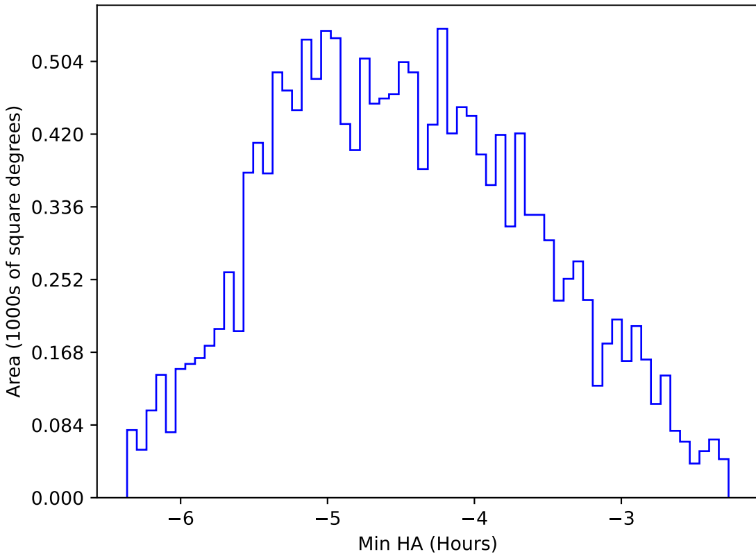
too_elab_r128_d3_gz_v3.4_10yrs WFD r band: Min HA
