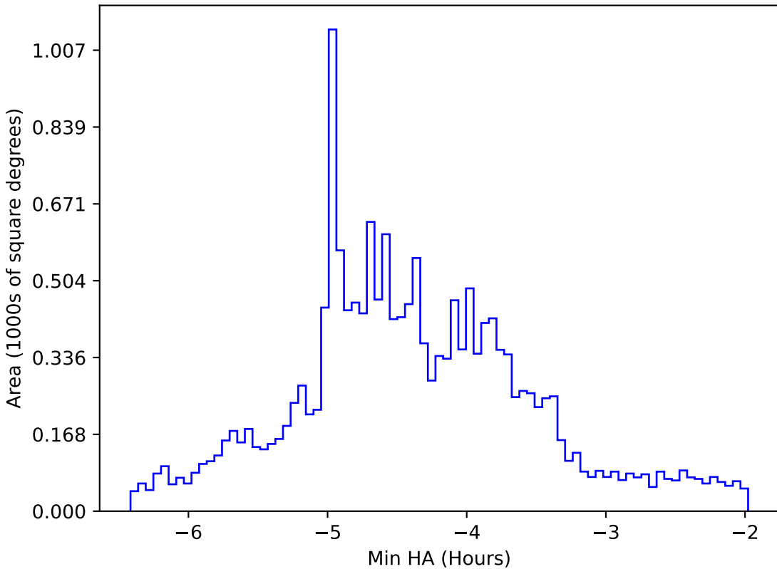
too_elab_r128_d3_gz_v3.4_10yrs WFD g band: Min HA
