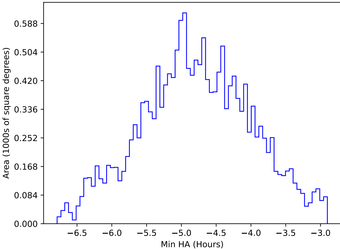
too_elab_r128_d3_gz_v3.4_10yrs WFD all bands: Min HA
