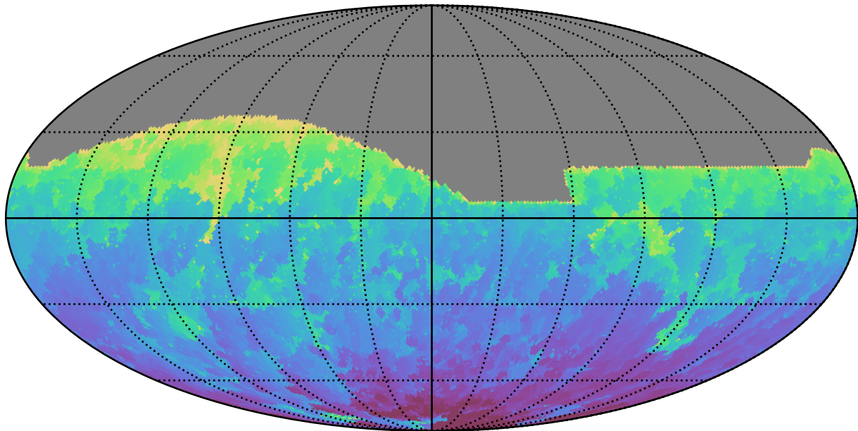
too_elab_r128_d3_gz_v3.4_10yrs All sky z band: Min HA
