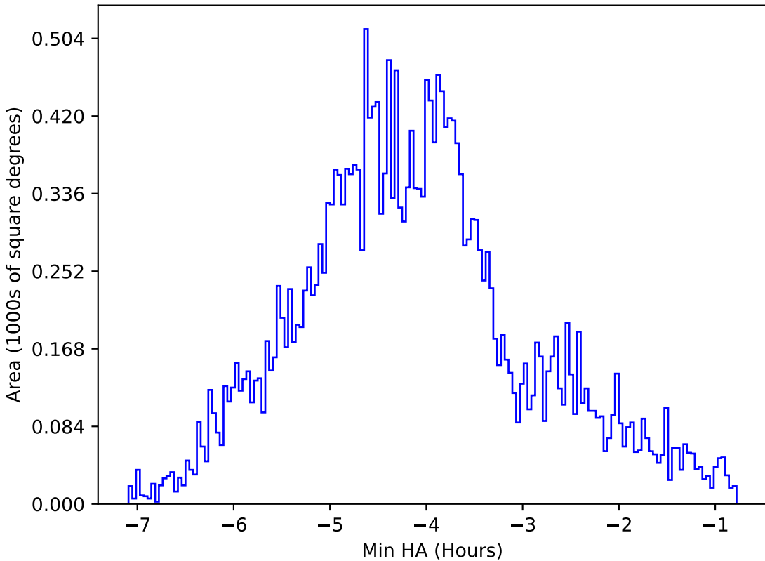
too_elab_r128_d3_gz_v3.4_10yrs All sky z band: Min HA
