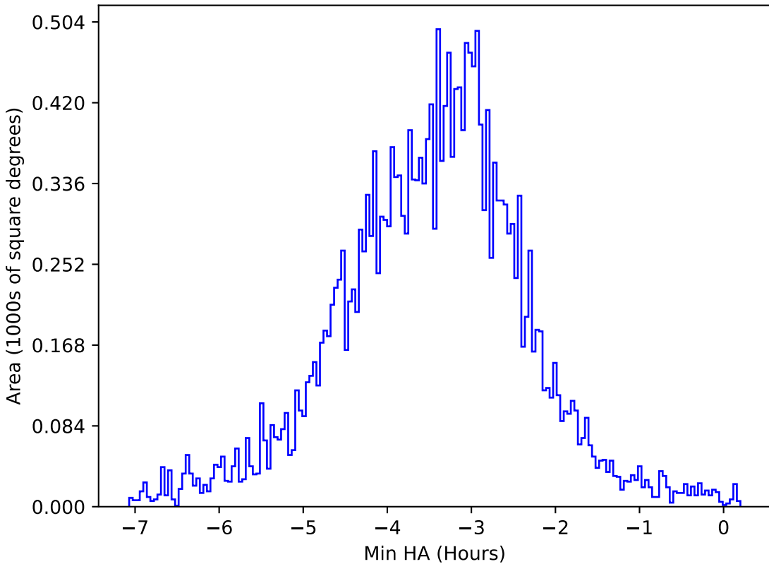
too_elab_r128_d3_gz_v3.4_10yrs All sky y band: Min HA
