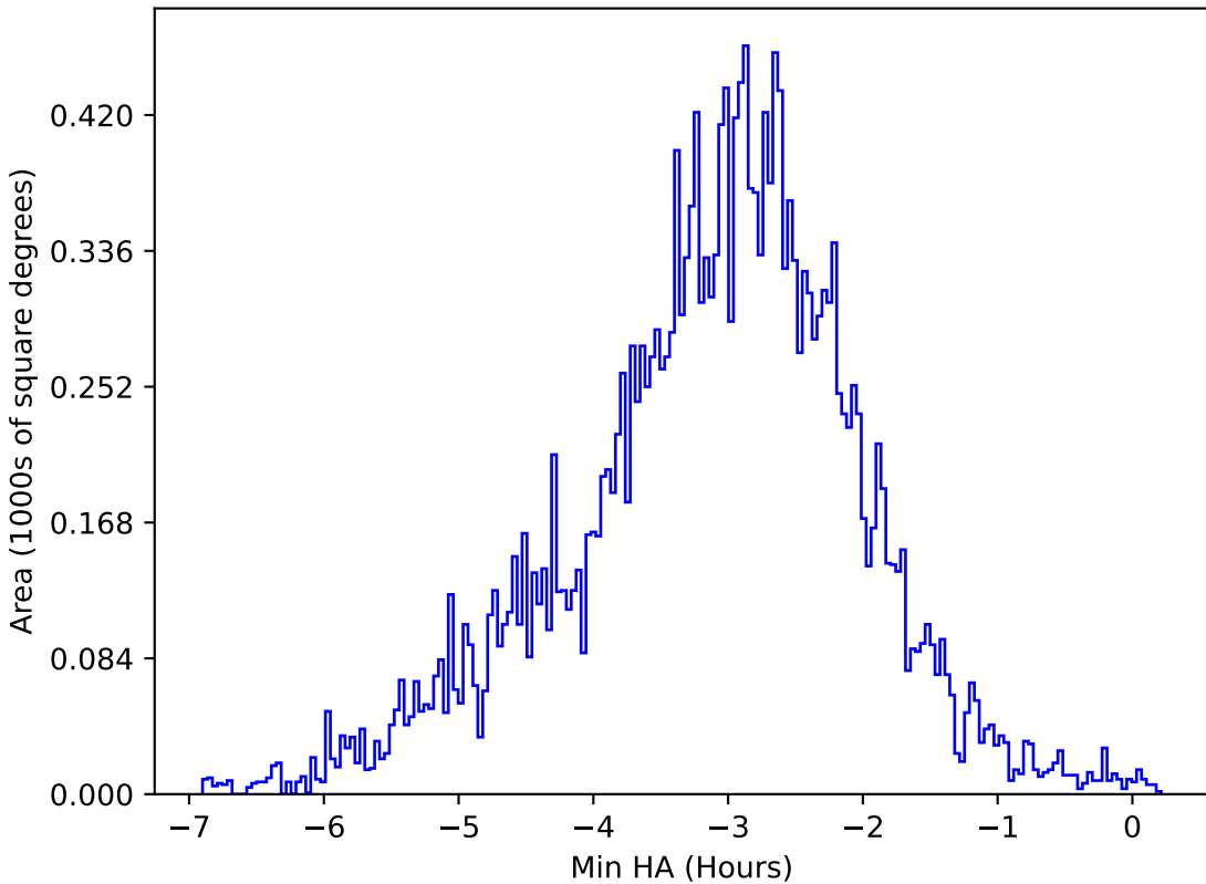
too_elab_r128_d3_gz_v3.4_10yrs All sky u band: Min HA
