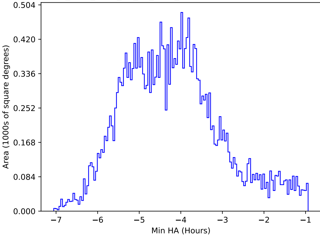
too_elab_r128_d3_gz_v3.4_10yrs All sky r band: Min HA
