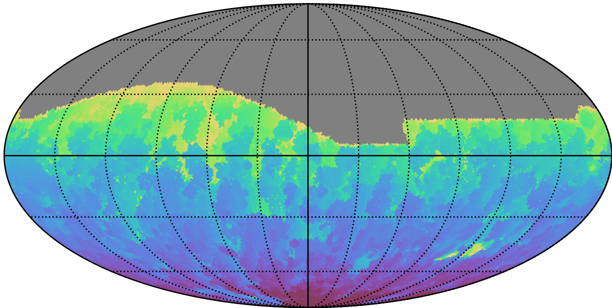
too_elab_r128_d3_gz_v3.4_10yrs All sky g band: Min HA
