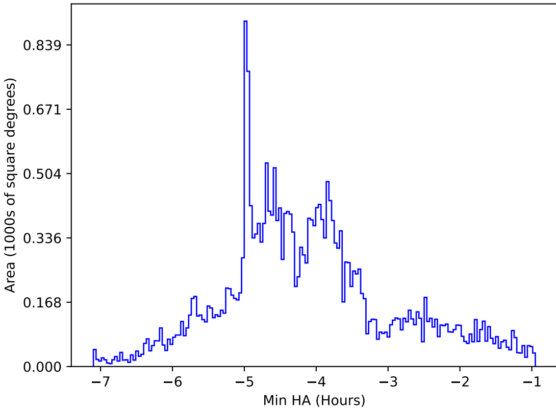
too_elab_r128_d3_gz_v3.4_10yrs All sky g band: Min HA
