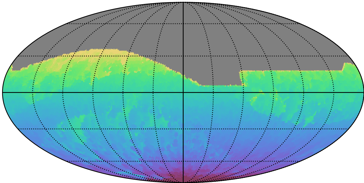
too_elab_r128_d3_gz_v3.4_10yrs All sky all bands: Min HA
