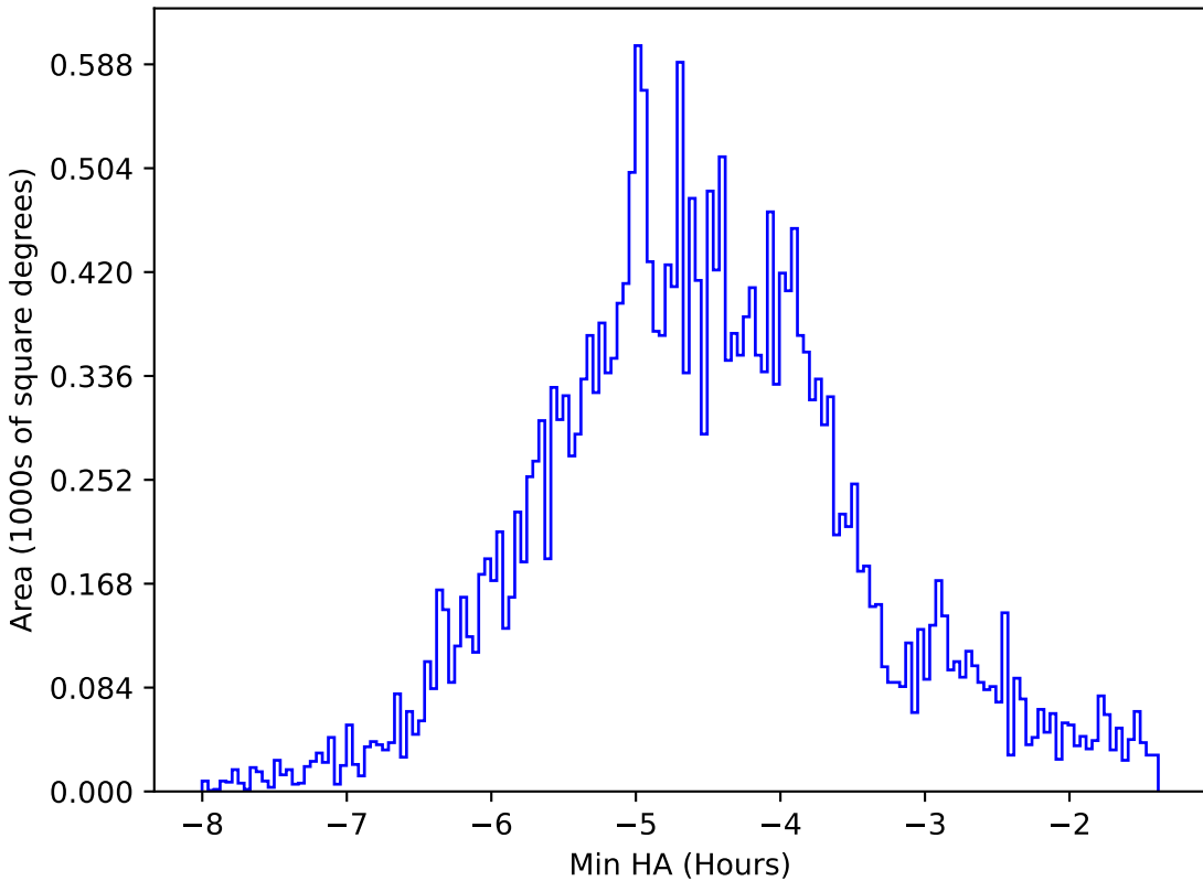
too_elab_r128_d3_gz_v3.4_10yrs All sky all bands: Min HA
