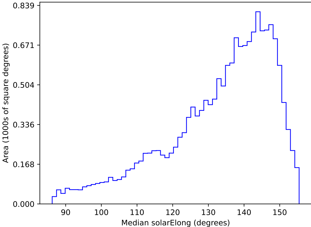
too_elab_r128_d3_gz_v3.4_10yrs WFD u band: Median solarElong
