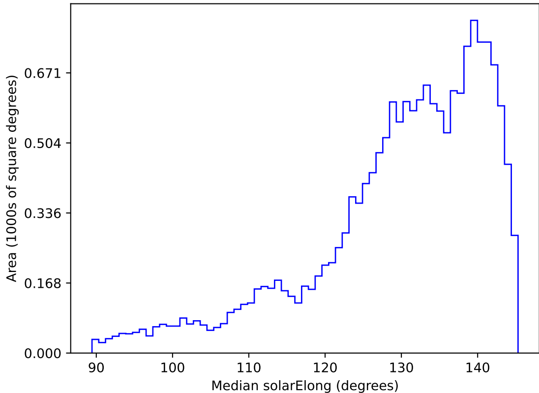
too_elab_r128_d3_gz_v3.4_10yrs WFD all bands: Median solarElong
