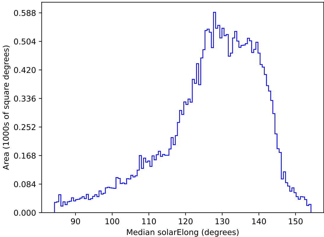
too_elab_r128_d3_gz_v3.4_10yrs All sky z band: Median solarElong
