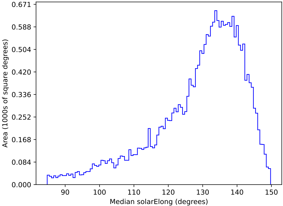
too_elab_r128_d3_gz_v3.4_10yrs All sky y band: Median solarElong
