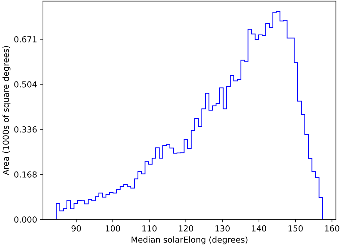
too_elab_r128_d3_gz_v3.4_10yrs All sky u band: Median solarElong
