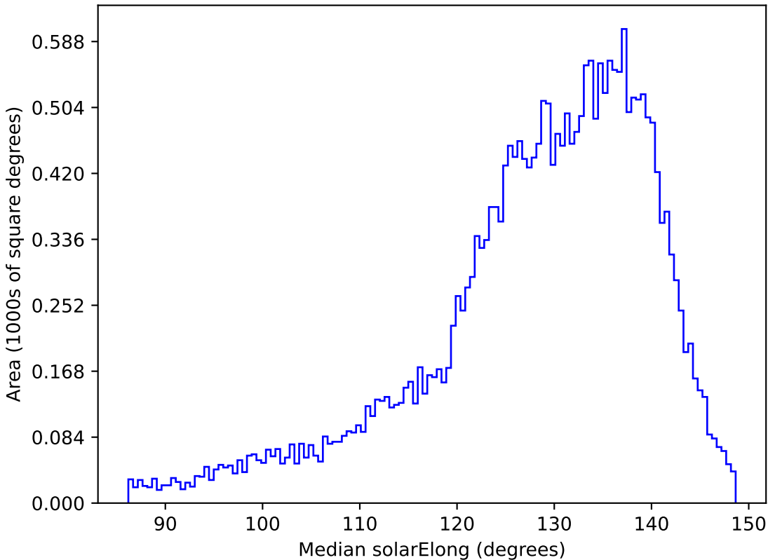
too_elab_r128_d3_gz_v3.4_10yrs All sky i band: Median solarElong
