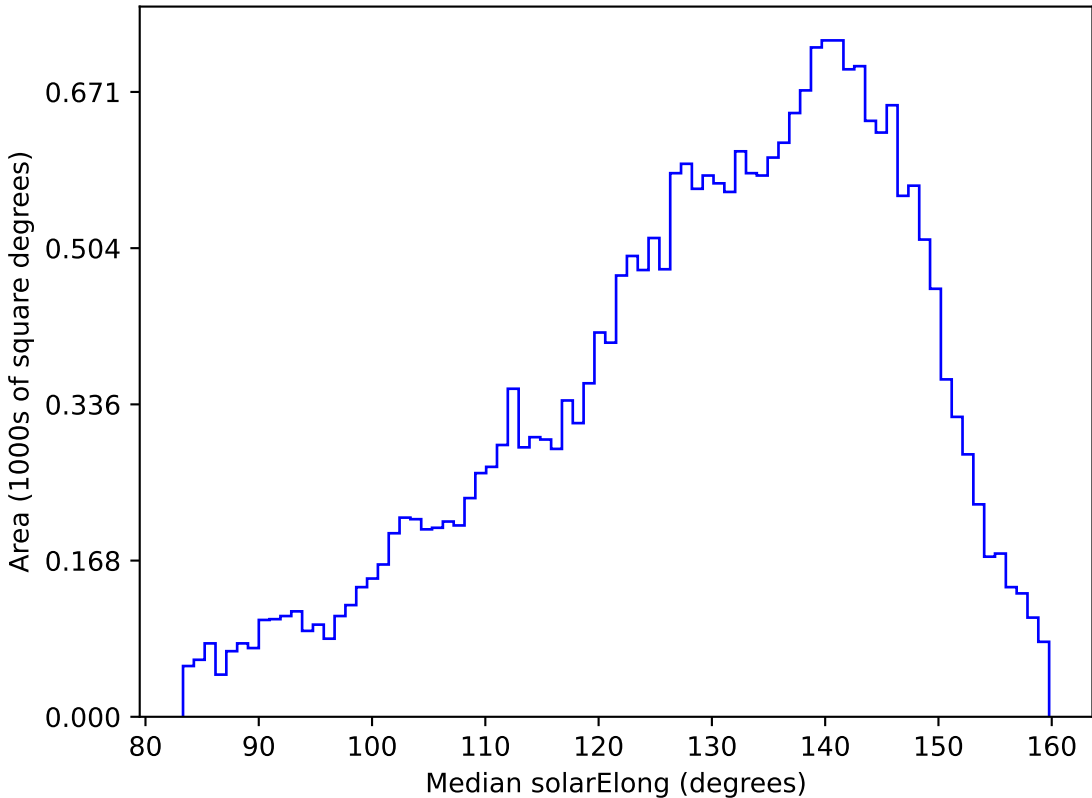
too_elab_r128_d3_gz_v3.4_10yrs All sky g band: Median solarElong
