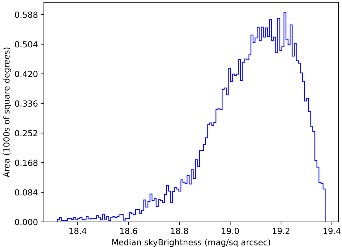
too_elab_r128_d3_gz_v3.4_10yrs Yr 1 z band: Median skyBrightness
