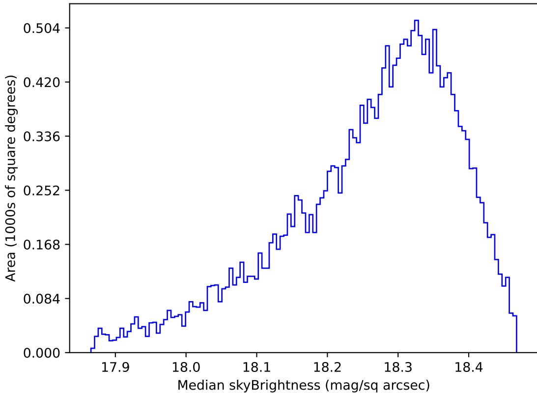
too_elab_r128_d3_gz_v3.4_10yrs Yr 1 y band: Median skyBrightness
