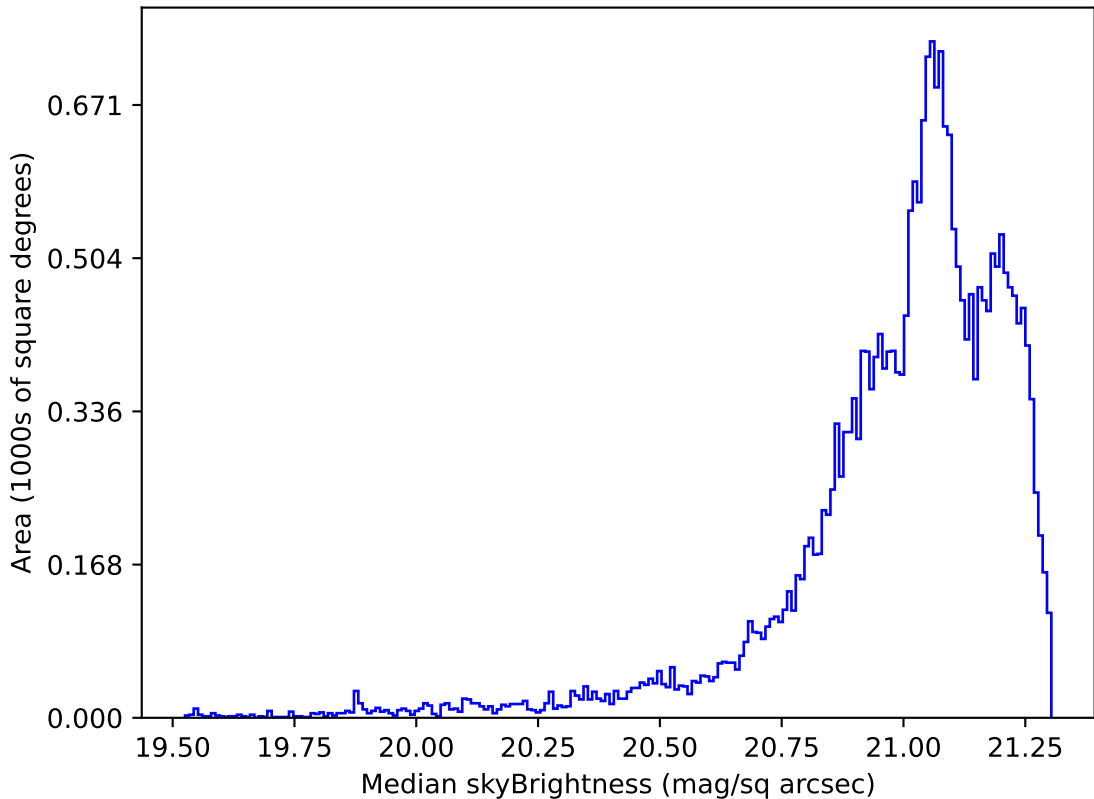
too_elab_r128_d3_gz_v3.4_10yrs Yr 1 r band: Median skyBrightness
