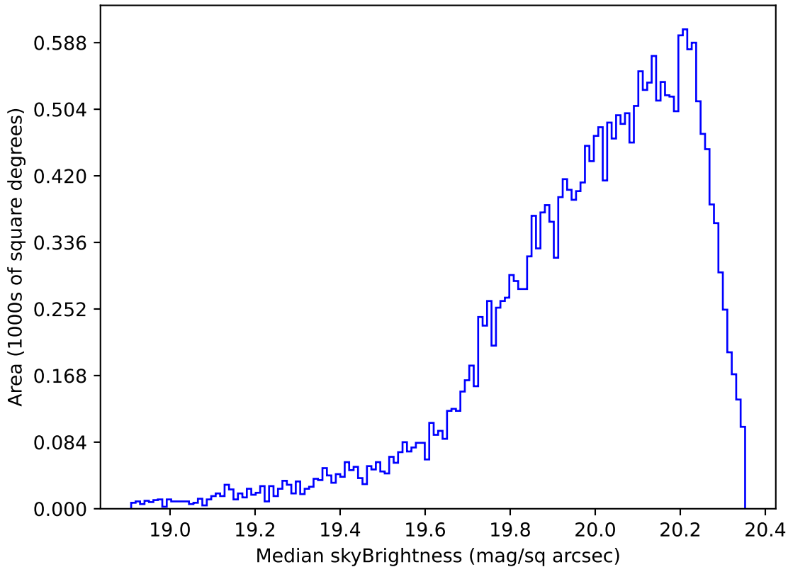
too_elab_r128_d3_gz_v3.4_10yrs Yr 1 i band: Median skyBrightness
