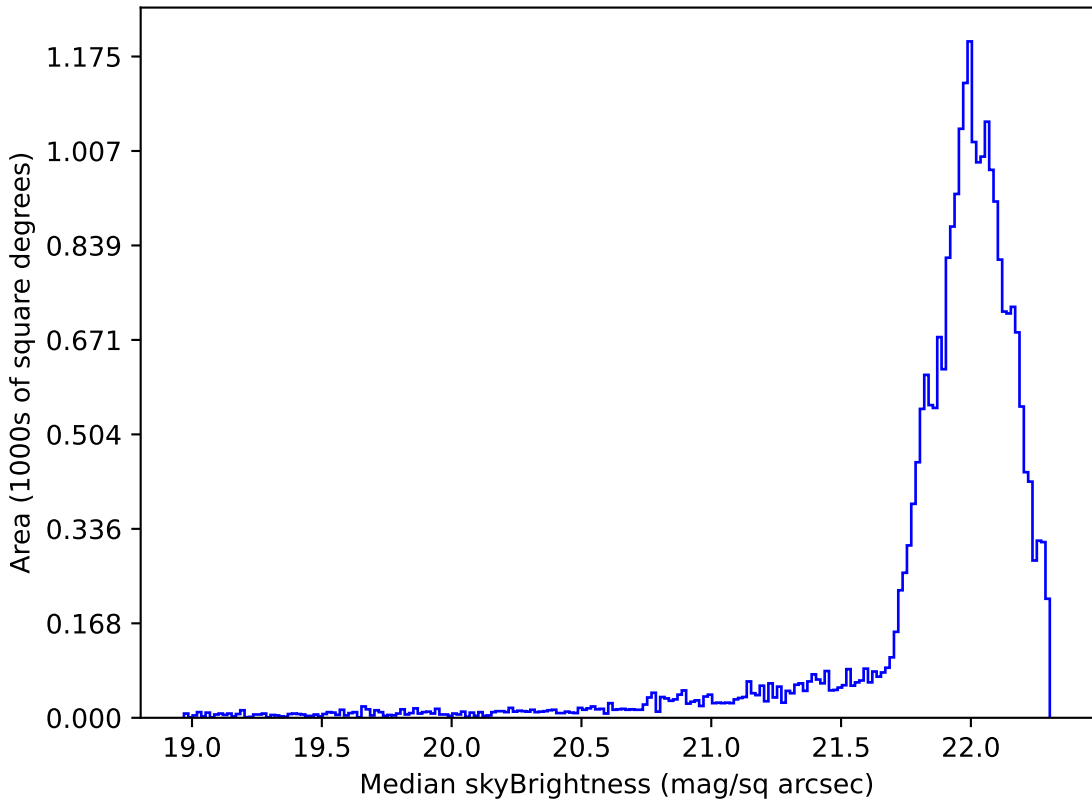
too_elab_r128_d3_gz_v3.4_10yrs Yr 1 g band: Median skyBrightness
