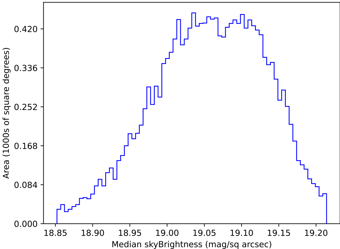
too_elab_r128_d3_gz_v3.4_10yrs WFD z band: Median skyBrightness
