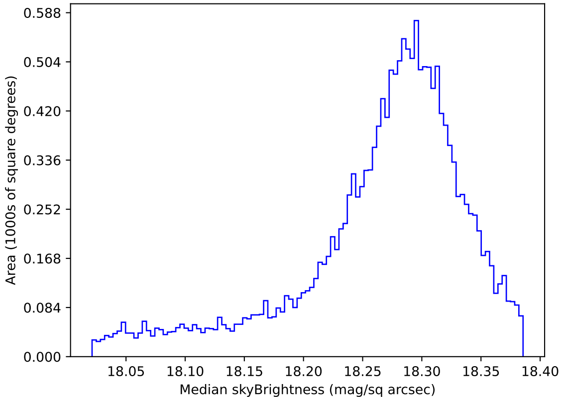
too_elab_r128_d3_gz_v3.4_10yrs WFD y band: Median skyBrightness
