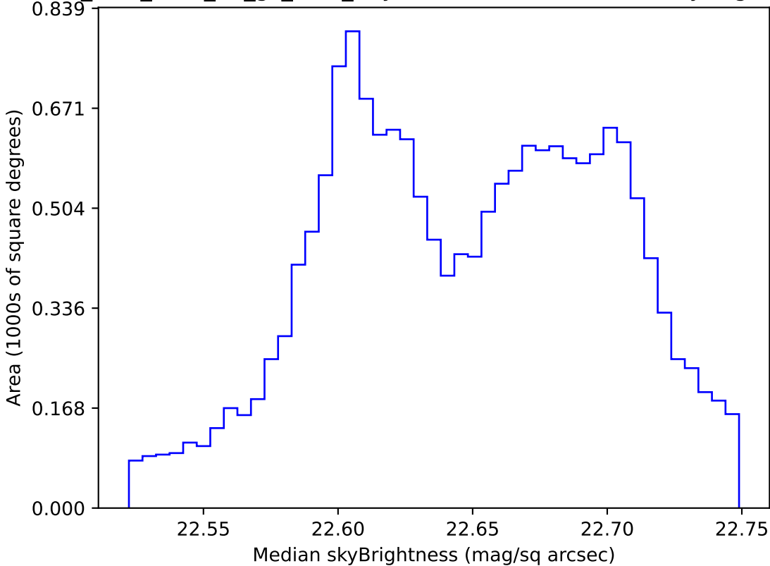
too_elab_r128_d3_gz_v3.4_10yrs WFD u band: Median skyBrightness
