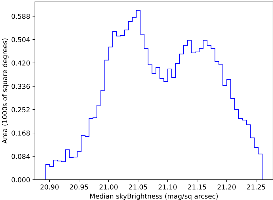
too_elab_r128_d3_gz_v3.4_10yrs WFD r band: Median skyBrightness
