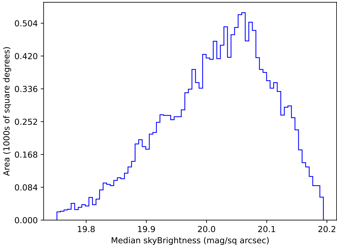
too_elab_r128_d3_gz_v3.4_10yrs WFD i band: Median skyBrightness
