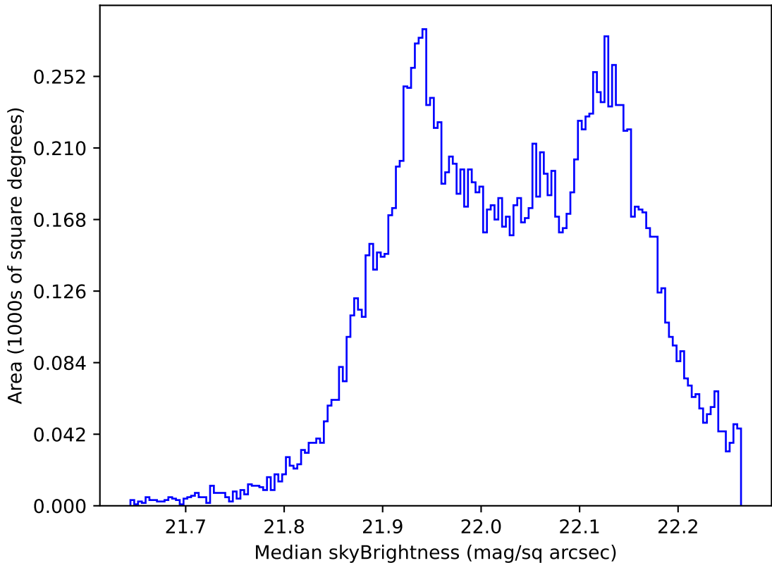
too_elab_r128_d3_gz_v3.4_10yrs WFD g band: Median skyBrightness
